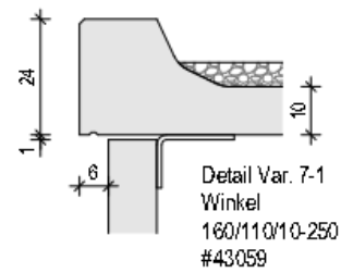
Dach "DV" Detail M 1 : 10
